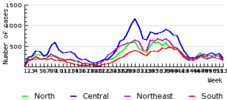
Number of HFM cases by week of onset and region.
