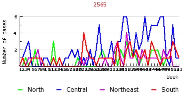
Number of Measles cases by week of onset and region.
