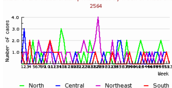
Number of L.G.V.&other&unsp.V.D. cases by week of onset and region
